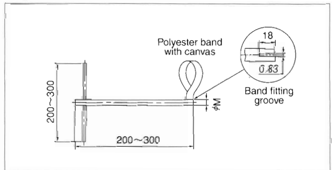
<Fig. G-16> Twist bar (Metal and Polyester band with canvas)
