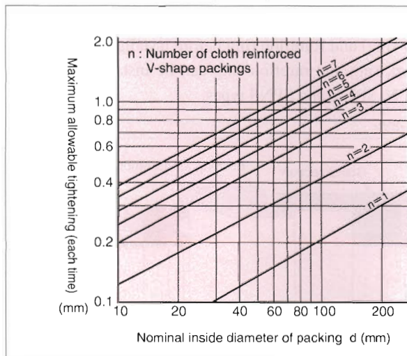
<Fig. G-32> Max. allowable tightening
